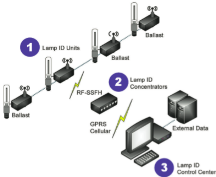
Menolinx Lighting Control Outdoor Solutions Triple Layer Architecture
